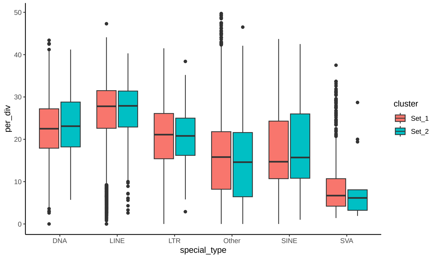
Divergence from overlapping TE H3K36me3 1bp
